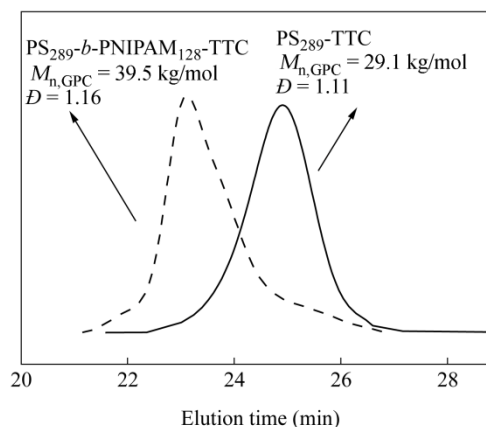
Fig. 1 The GPC traces of the PS 289 -TTC and PS 289 - b -PNIPAM 128 -TTC macro-RAFT agents
