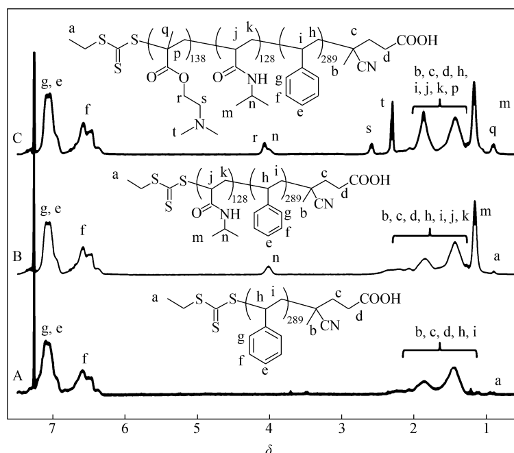
Fig. 2 The ^1\text{H} -NMR spectra of the PS 289 -TTC (A), PS 289 - b -PNIPAM 128 -TTC (B) macro-RAFT agents, and PS 289 - b -PNIPAM 128 - b -PDMAEMA 138 triblock copolymer (C)
